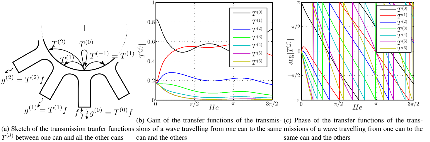
FIGURE 9: a) Sketch of the reflection/transmission transfer functions T^{(d)} for an in-coming travelling wave f . Each function T^{(d)}(\omega) is the transmitted Riemann invariant from one can to a can that is d cans apart. For example T^{(0)} is the reflection of a wave propagating downstream of one can and being reflected to the same can, and T^{(3)} can be interpreted for example as the transmission of a wave travelling downstream can 4 and propagating upstream in can 7, or any other two cans that are 3 cans apart. b,c) Gain and phase of the transfer functions T^{(d)} between all cans.
