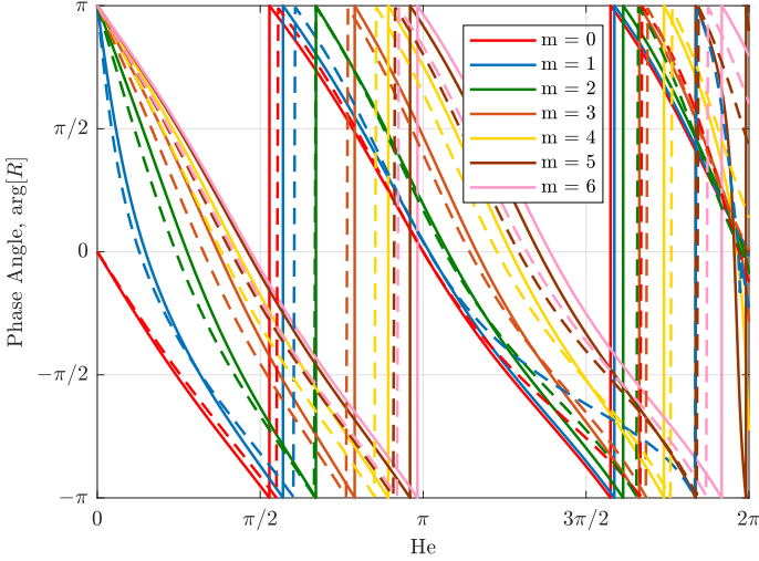
FIGURE 6: Validation of the geometrical simplifications for the 2D model for N = 12 . The dashed lines are obtained from a fixed complex 3D geometry, while the continuous lines are obtained with the bidimensional model proposed in this manuscript, with the nondimensional values estimated from the 3D geometry without applying further corrections. The good agreement validates the geometrical approximations made to map the complex 3D geometry to the simpler 2D model.
