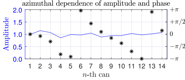
(a) second azimuthal mode m = 2
