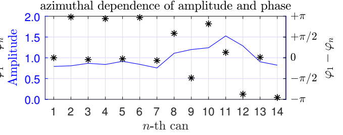
(b) push-pull mode m = N/2 = 7
