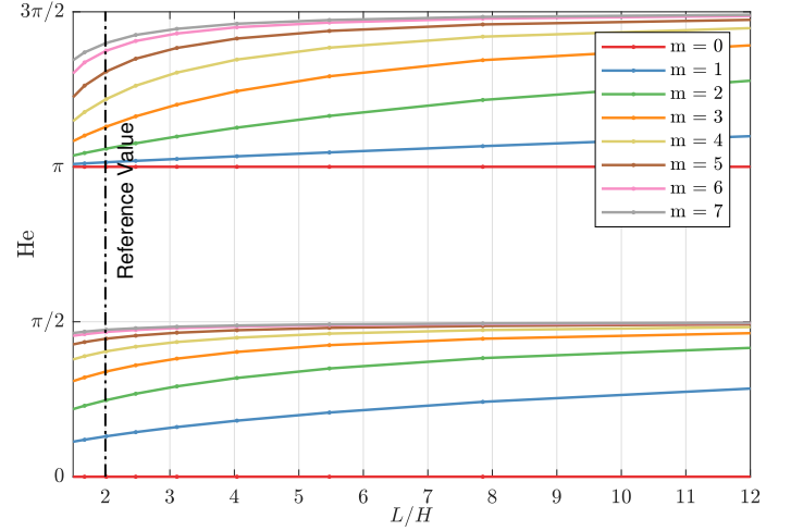
FIGURE 7: Sensitivity of the first two eigenfrequencies of a can system as function of the geometry aspect ratio L/H , for all azimuthal wavenumber m , for N = 14 . We plot the Helmholtz number of all the eigenmodes with He < 2\pi for each azimuthal mode m , as function of the two nondimensional parameters governing can to can acoustic communication. As L/H increases, the Helmholtz number of the azimuthal modes converge slowly to \pi/2 and 3\pi/2 for the first two modes. For a fixed value of L/H , the eigenfrequencies for m = 5, 6, 7 are rather close, forming a cluster. These modes are closer together the larger is L/H .
