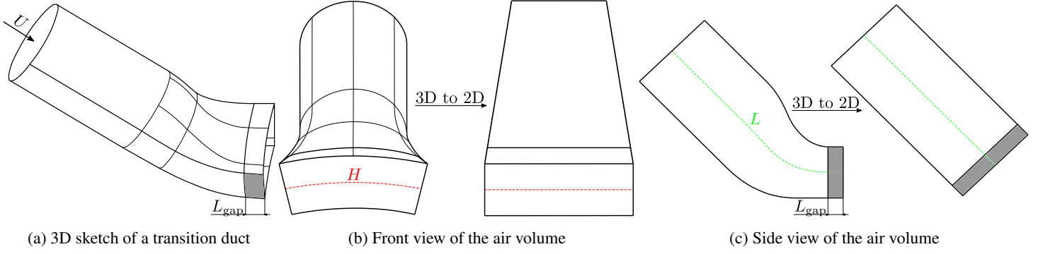
FIGURE 1: Geometry of a typical transition duct and the simplifications leading to the 2D model, appearing ultimately in Fig. 2a. The communicating gap between two adjacent transition ducts is colored in gray, with an axial length L_{\text{gap}} .
