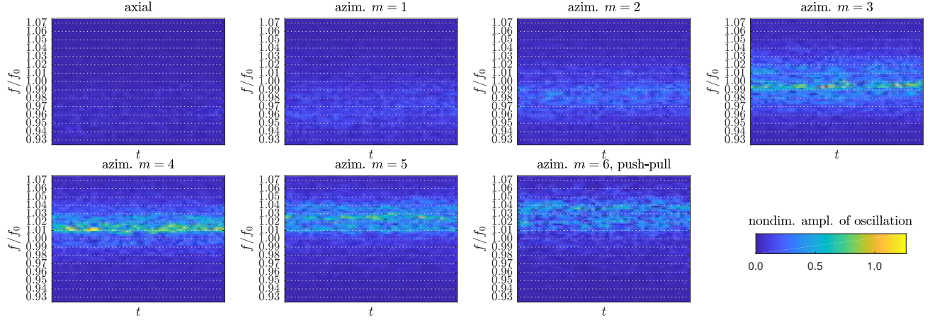
FIGURE 8: Spectrogram of the timeseries of the azimuthal modes reconstructed from an engine. We can observe that more than one azimuthal mode is active in a small range of frequencies, forming a cluster. Within the cluster, each mode peaks at a frequency that increases with the azim. order m . The highest amplitude is not always in the same mode, and the system's energy appears to move randomly between the modes, with some statistical preference for the m = 3, 4, 5 modes.
