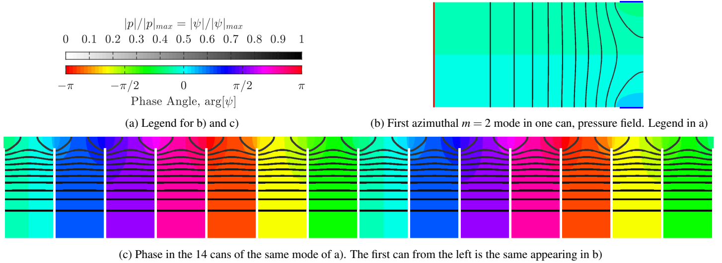
FIGURE 3: First eigenmode with azimuthal order m = 2 , for a set of N = 14 communicating cans. Because the solution is complex-valued, we use different colormaps for the absolute value and the phase angle, presented in the two legends in a). In b) we present the solution in one can only: we observe that the phase is approximately constant on the cross section at the upstream end of the transition duct, on the left, far from the cross-talk area. The amplitude decreases slightly from left to right. In c) we present the ensemble of all the 14 cans pulsating together for the mode in b), reconstructed using (1). The phase changes mostly at the cross-talk area, and changes 2 times (since the azimuthal order m is 2) the quantity 2\pi along the annulus. At the upstream end of each transition duct the phase is approximately constant and the mode presents a certain azimuthal phase pattern. The phase between two cans is the difference of the phase value between two locations. Refer to Fig. 4a for experimental evidence of a second order azimuthal mode like this one in an engine.
