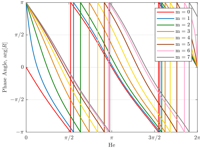
FIGURE 5: Phase of the equivalent reflection coefficient for the azimuthal modes for N = 14 cans, calculated with reference cross-section at the red inlet of the transition duct of Fig. 2a. The Helmholtz number is defined as He = L\omega/c .
