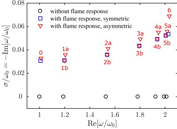
FIGURE 11: Complex eigenvalues for the three cases considered. The eigenvalues have been normalized with the angular eigenfrequency of the quarter-wave mode of an isolated can. The vertical axis is the normalized growth rate of oscillation of each mode. The red numbers refer to the asymmetric case and describe the m -th azimuthal order of the respective symmetric eigenmode. The amplitude and phase of each asymmetric mode is presented in Fig. 12 in the plot with the same red number in the top left corner.
