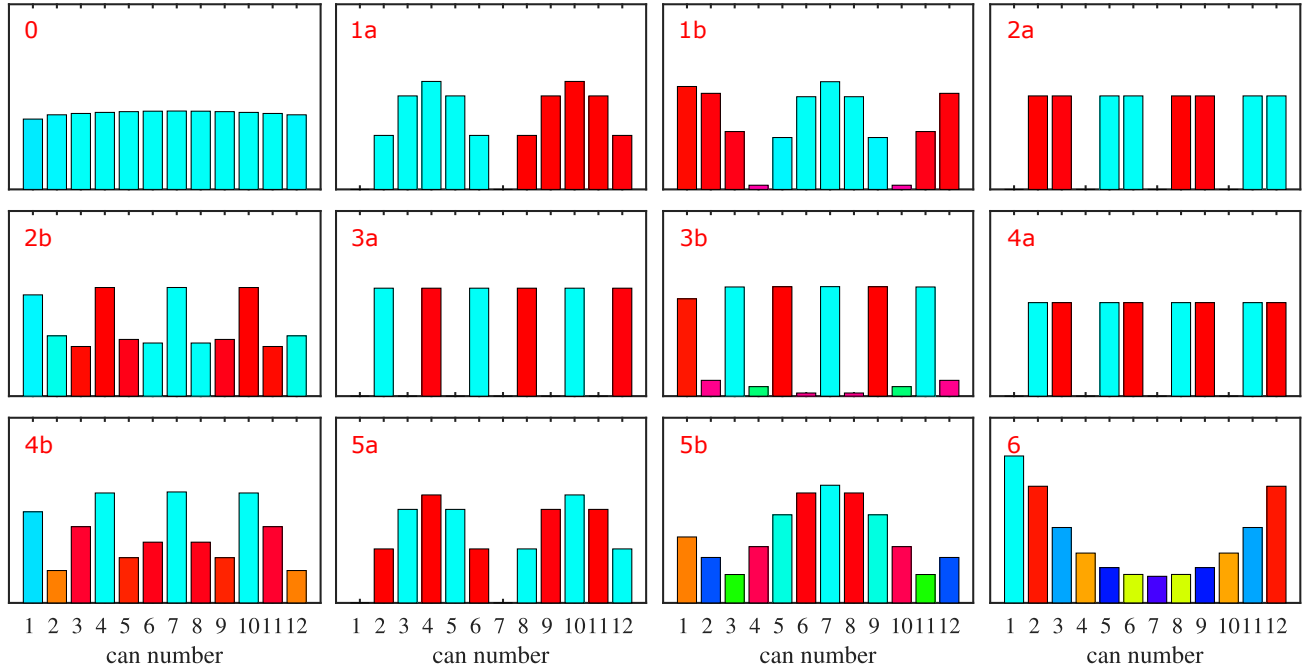
FIGURE 12: Visualization of the azimuthal mode shapes associated with the eigenvalues of the asymmetric case (Fig. 11). Ordered from left to right and top to bottom with increasing oscillation frequency. The bar height indicates the pressure amplitude and the bar color the phase (same color legend as in Fig. 3), at the interface between each can and each transition duct. The number in the top left corner is the azimuthal order m of the corresponding mode in the symmetric case. Couples of modes with the same m differ very little in frequency and can result in a slowly modulated linear combination with approximately constant amplitude along the annulus. This is not the case for the perturbed push-pull mode in the bottom right corner, where cans 1, 2, 3, 10, 11, 12 present much larger amplitude than the others.
