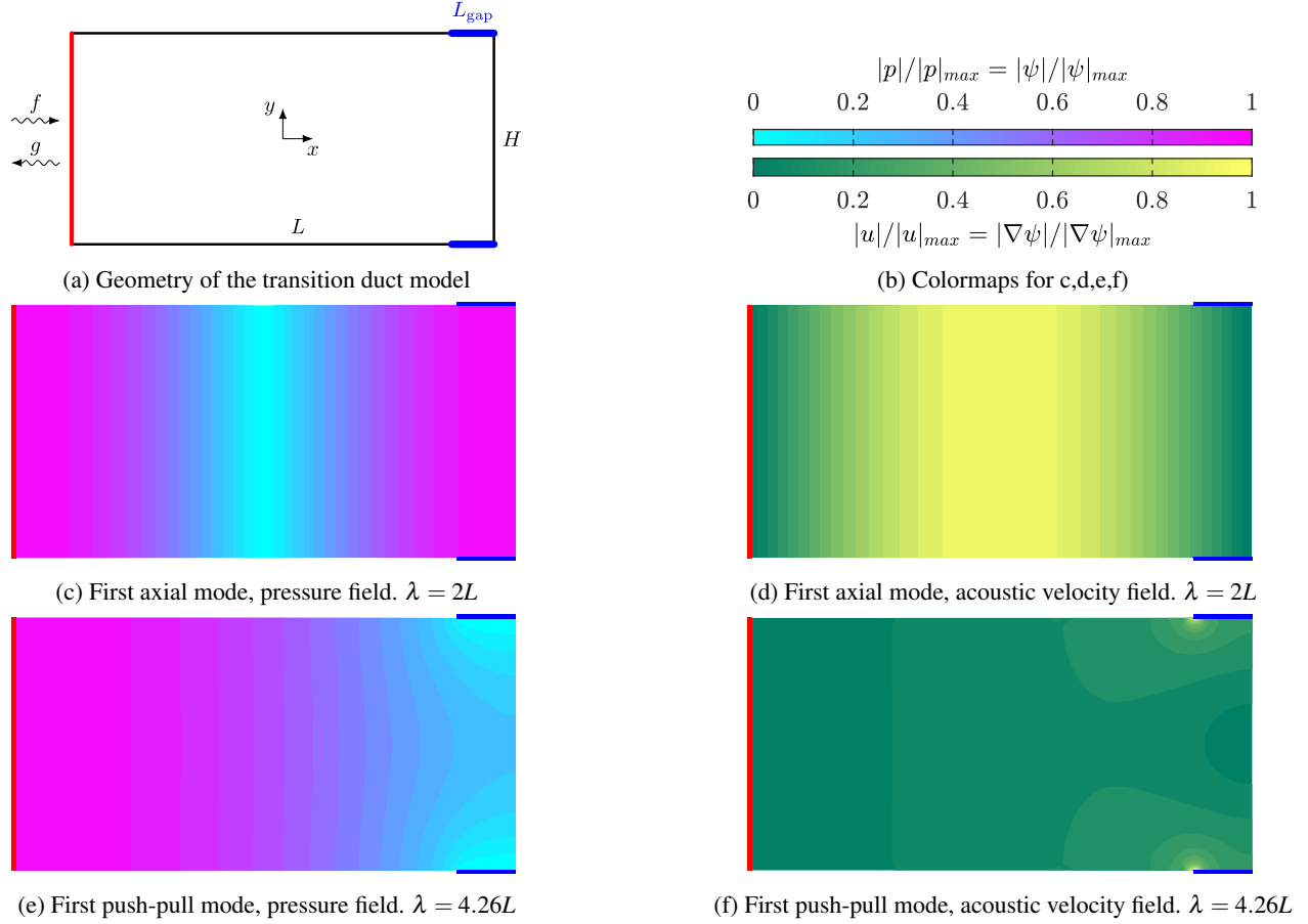
FIGURE 2: (a) geometry of the 2D model of the transition duct, simplified from the original geometry of Fig. 1. (b) legend, common to the other four figures. c) and d): first non-trivial eigenmode of the studied geometry for an axial mode, i.e. m = 0 . Absolute value of the acoustic pressure on the left, and absolute value of the acoustic velocity on the right. The solutions of the axial case match the solutions of the problem with Neumann conditions applied over the whole boundary. e) and f): same of c) and d) but for a push-pull mode, i.e. m = N/2 = 7 , for a set of N = 14 cans. In f) the acoustic velocity has a strong increase where the gap starts and is inhomogeneous over the gap length.
